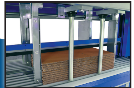
3-Sided Bundle Control
