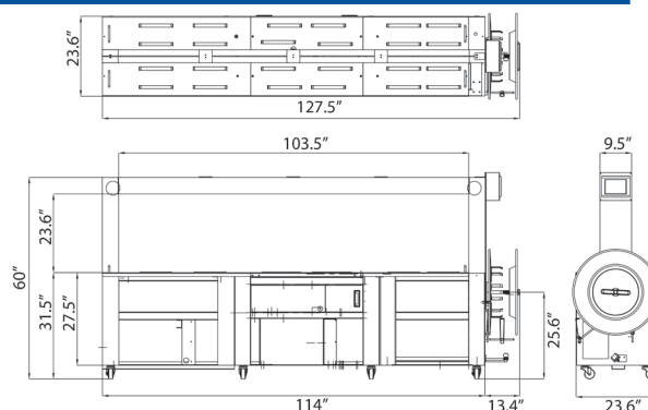
Width varies with arch size
