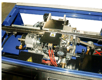
Powered by Servo Motors
