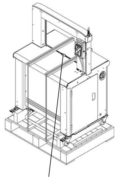
Center-of-gravity position
